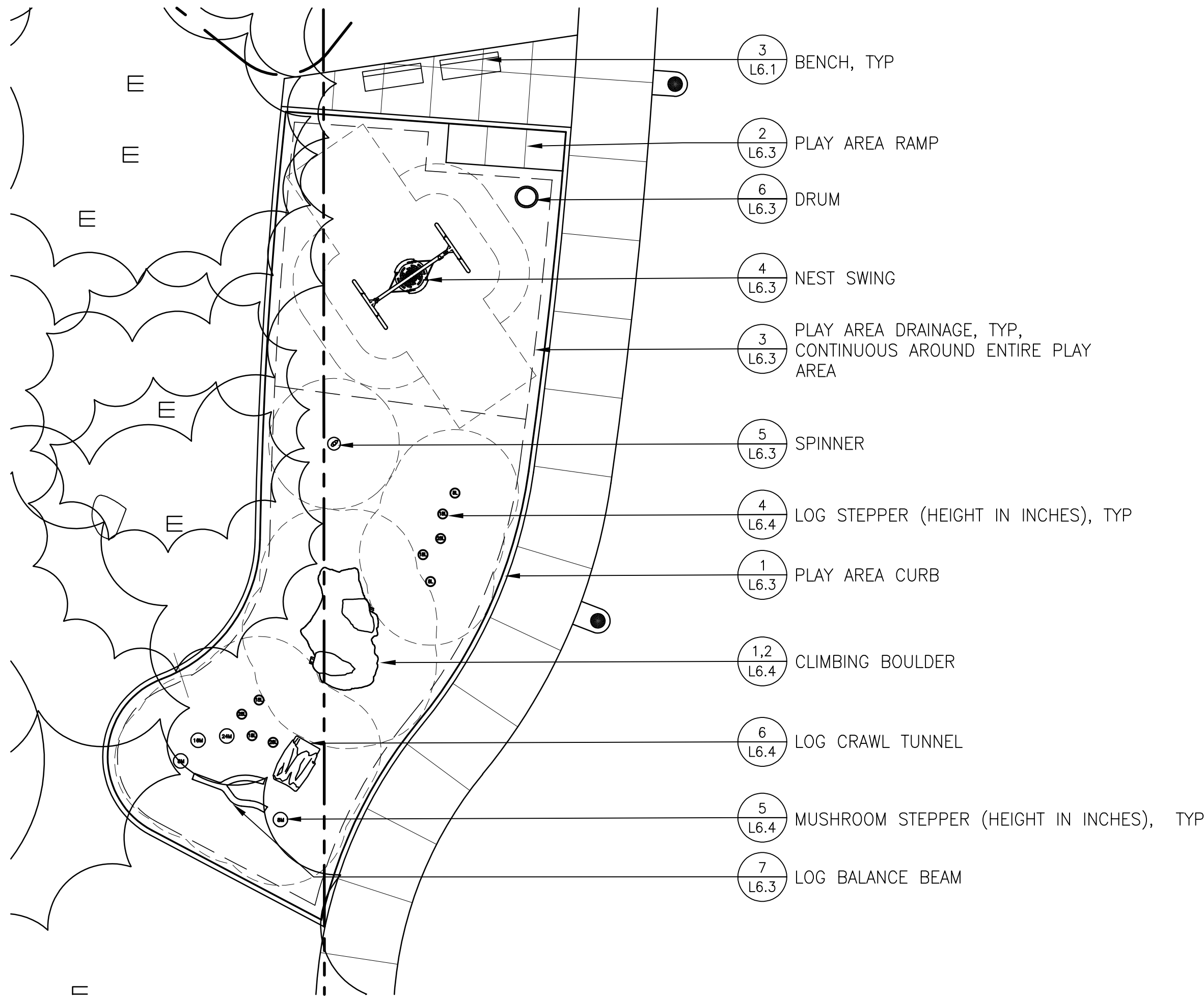
1 PLAY AREA - ENLARGED MATERIALS PLAN
