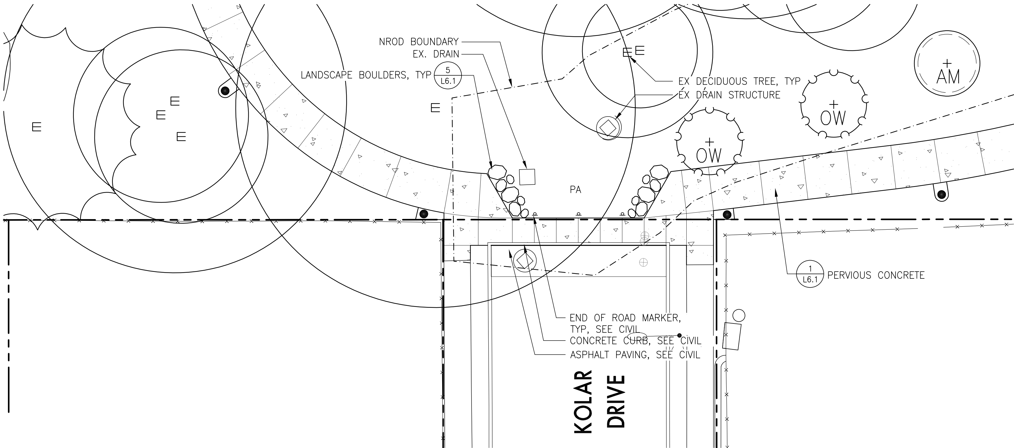
2 SOUTH ENTRY - ENLARGED MATERIALS PLAN
