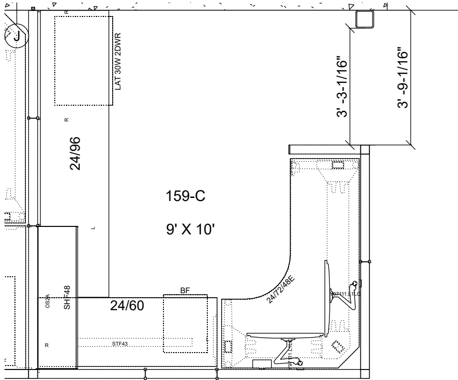
OPEN OFFICE Scale 3/8" = 1'
