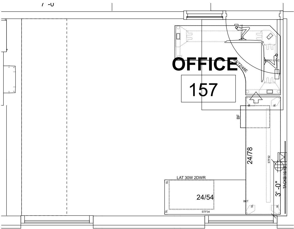
Scale 3/8" = 1'
