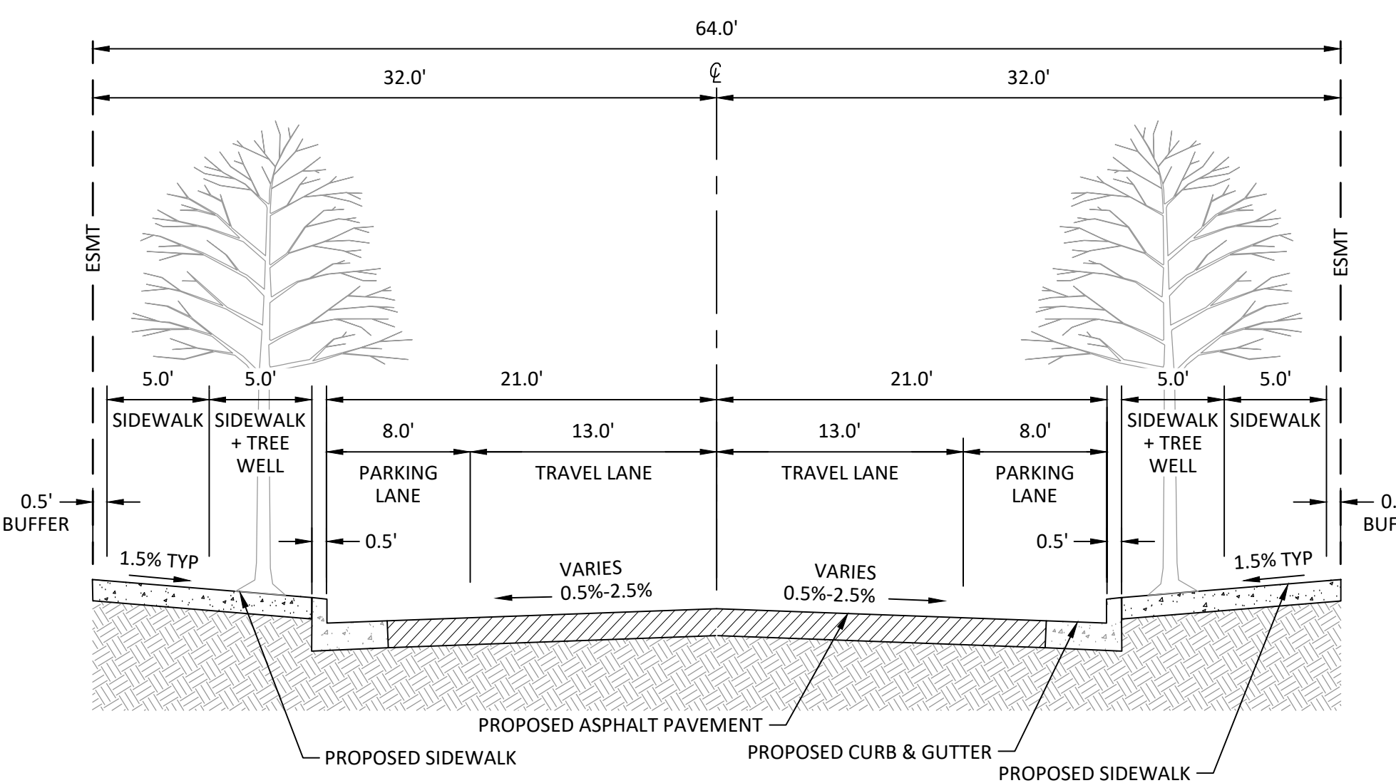
INTERNAL ROADS (W/ FIRE ACCESS) N.T.S.
