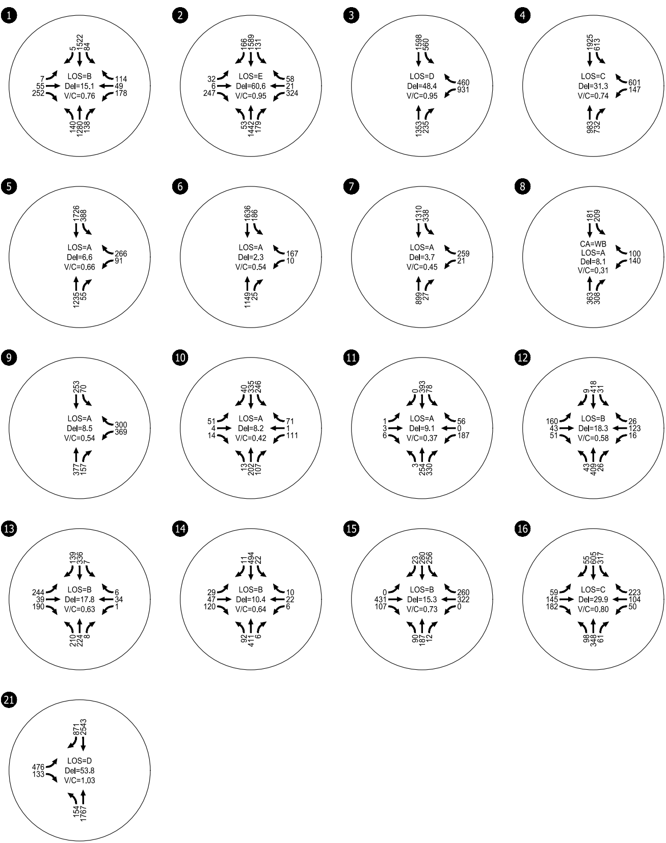
Year 2025 Background Traffic Conditions Weekday PM Peak Hour Oregon City, Oregon
