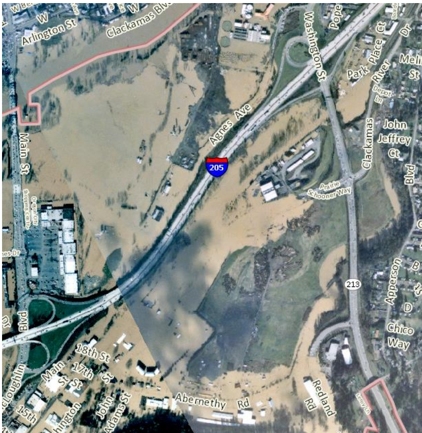
Figure 7 1996 Flood Inundation
