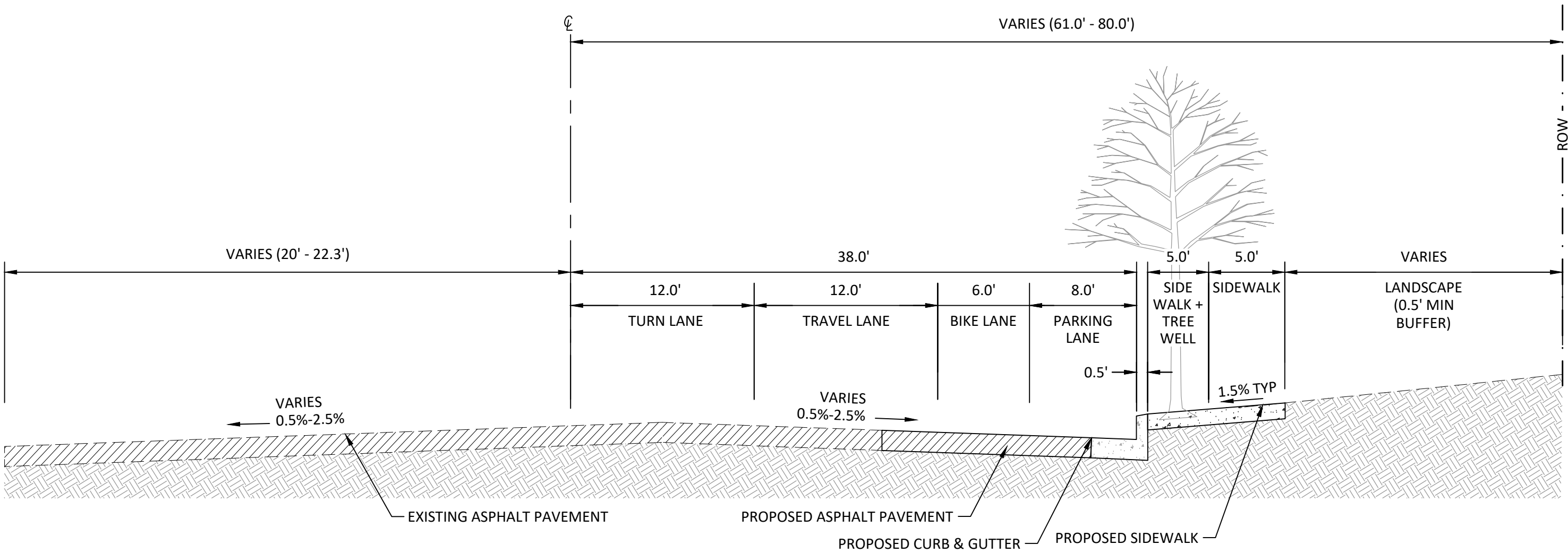
WASHINGTON STREET (HALF-STREET - 3 LANE) N.T.S.
