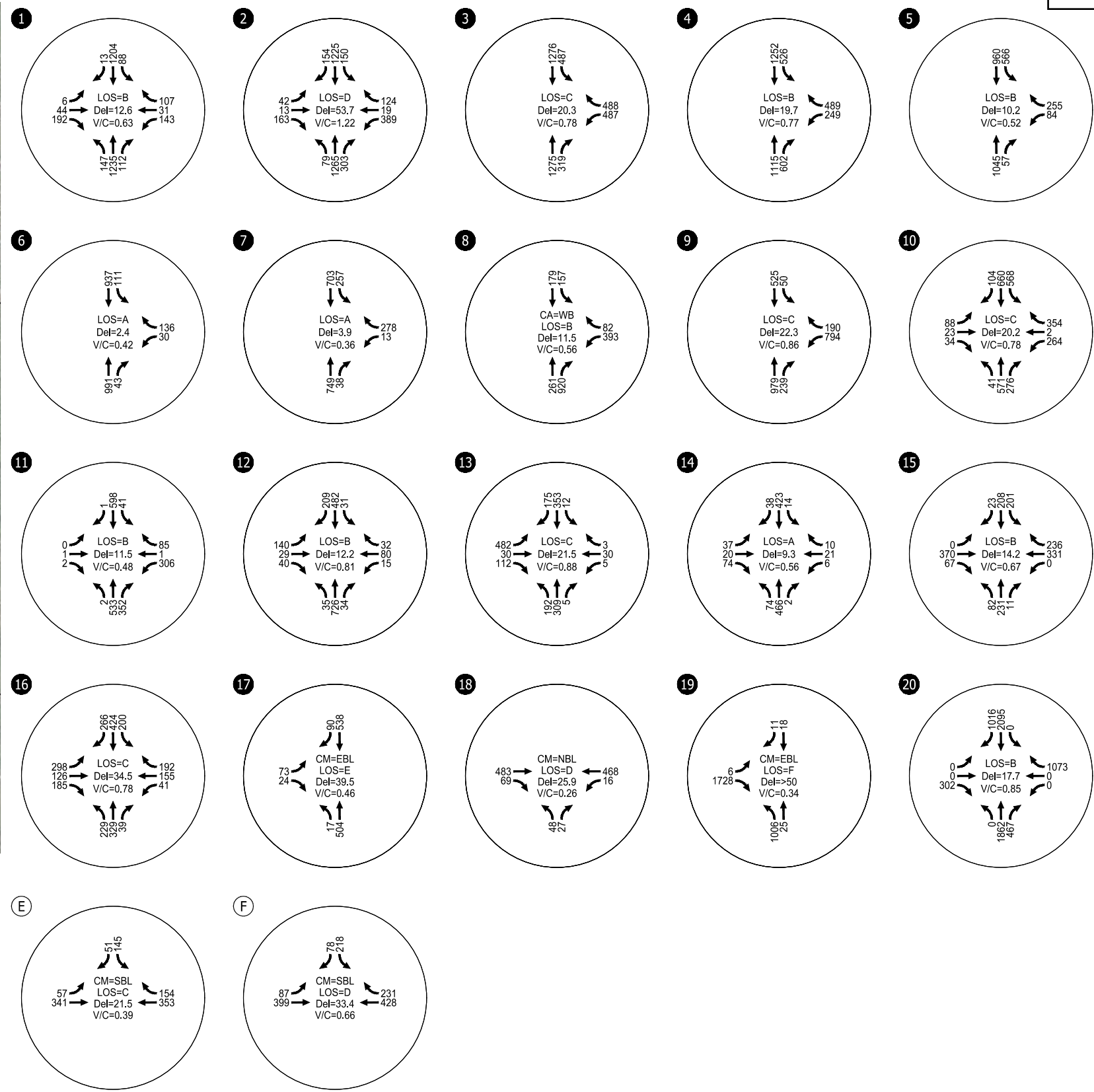
Year 2025 Total Traffic Conditions Saturday Midday Peak Hour Oregon City, Oregon
