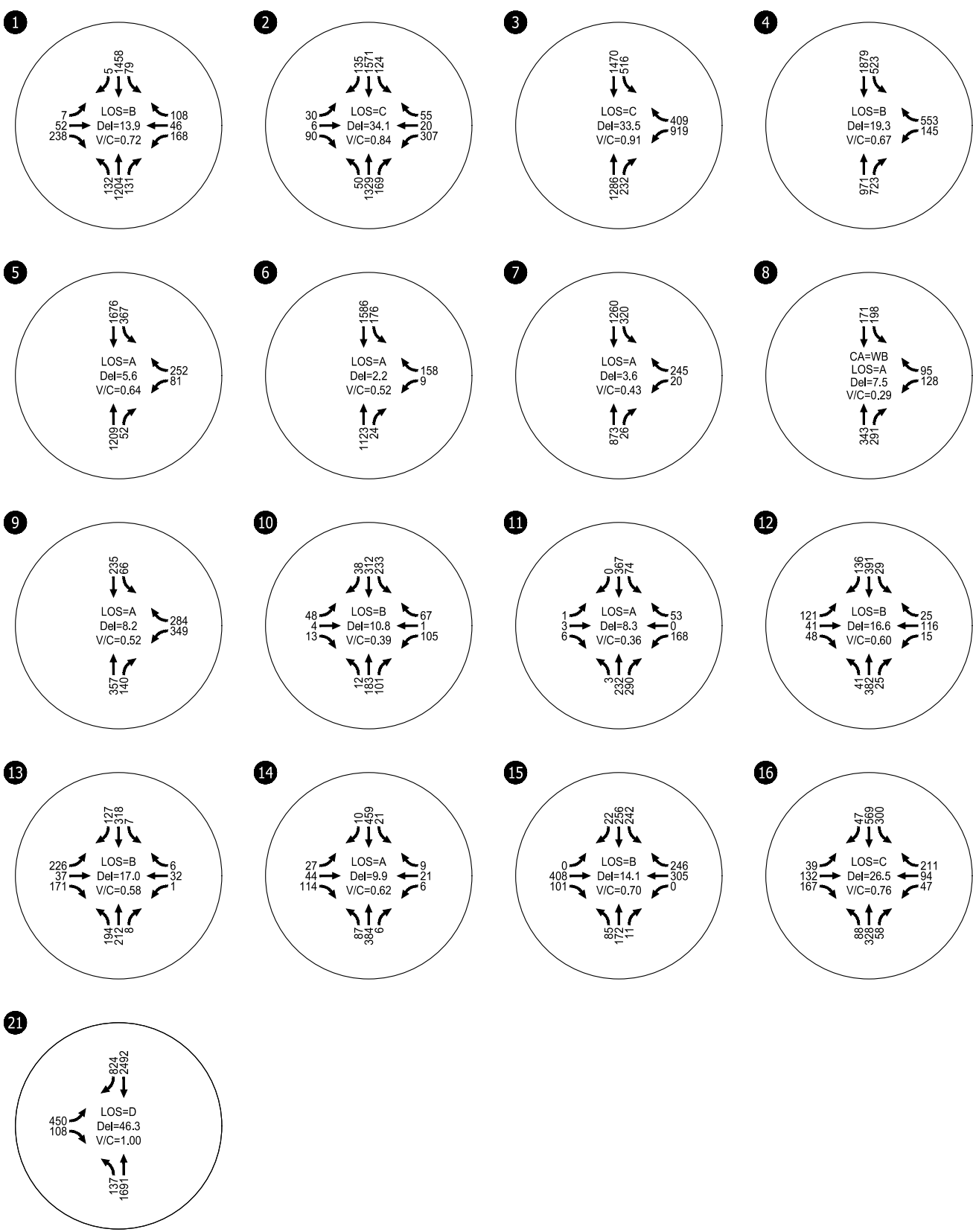
Estimated Existing Traffic Conditions Weekday PM Peak Hour Oregon City, Oregon Figure 8
