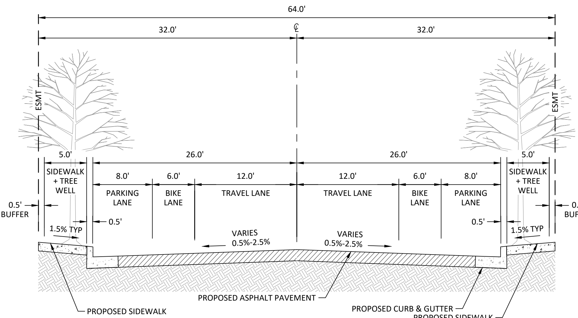
MARKET STREET (SECTION 3) N.T.S.
