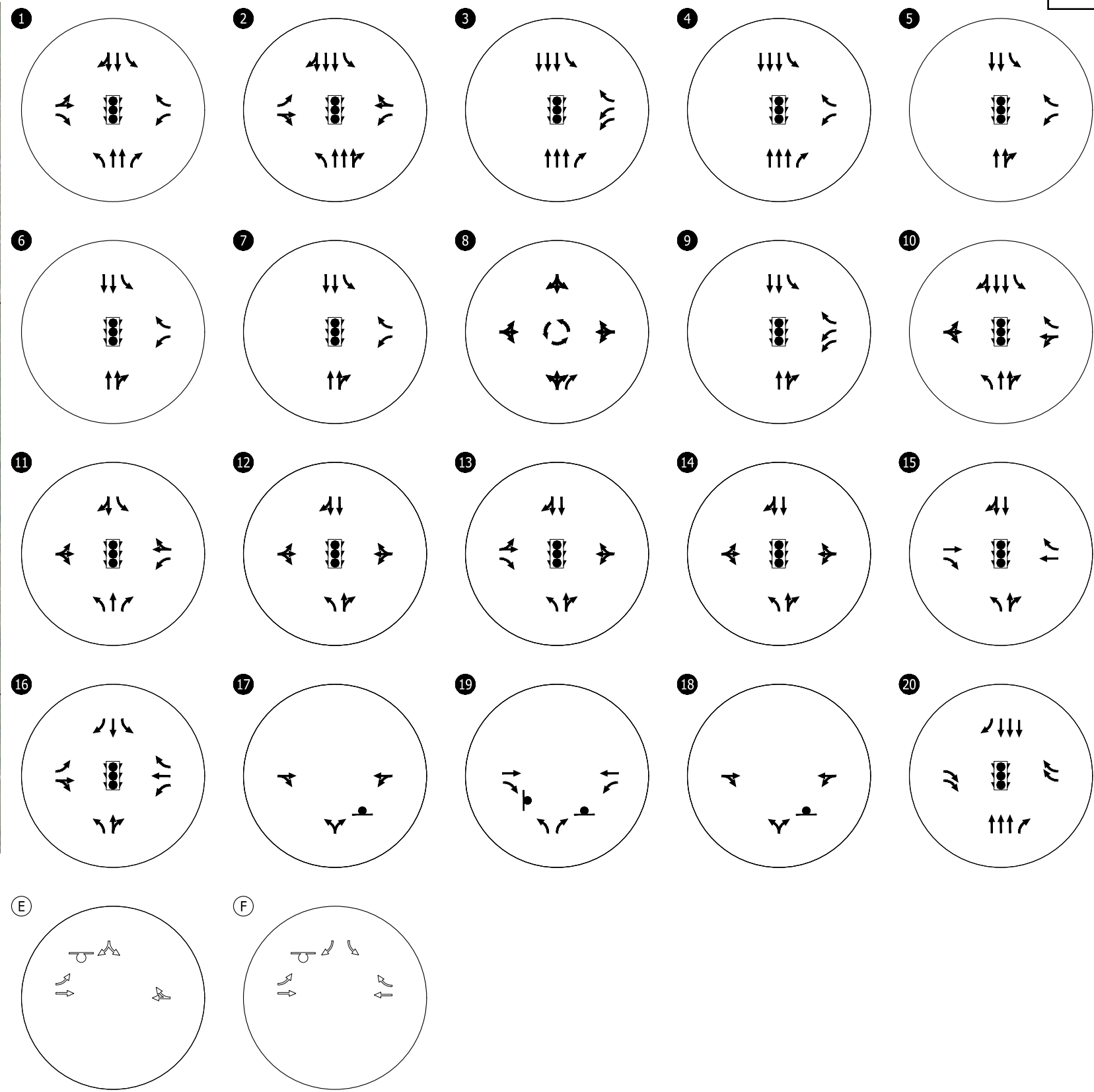
Assumed Lane Configurations & Traffic Control Devices Oregon City, Oregon
