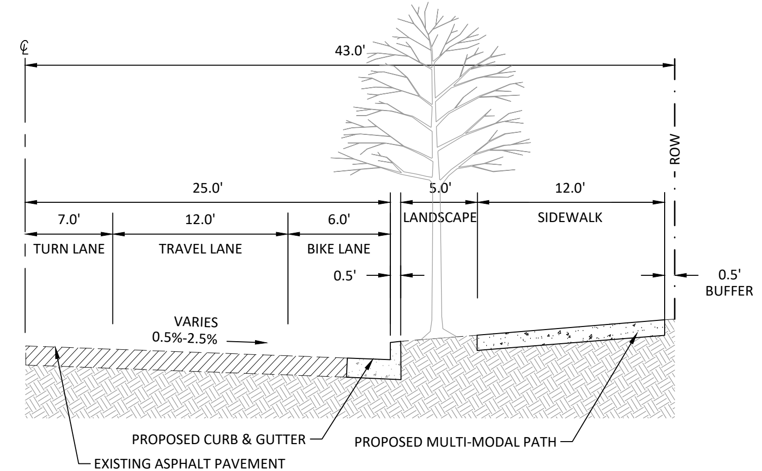
ABERNETHY ROAD (HALF-STREET) N.T.S.
