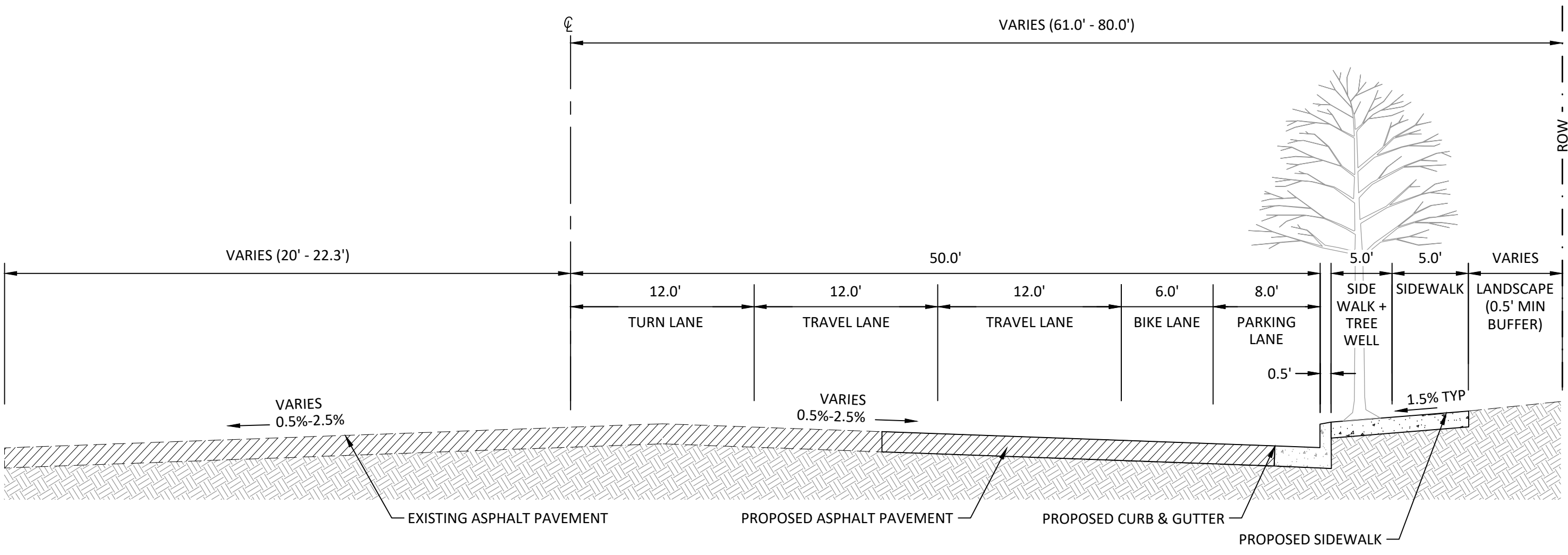
WASHINGTON STREET (HALF-STREET - 5 LANE) N.T.S.
