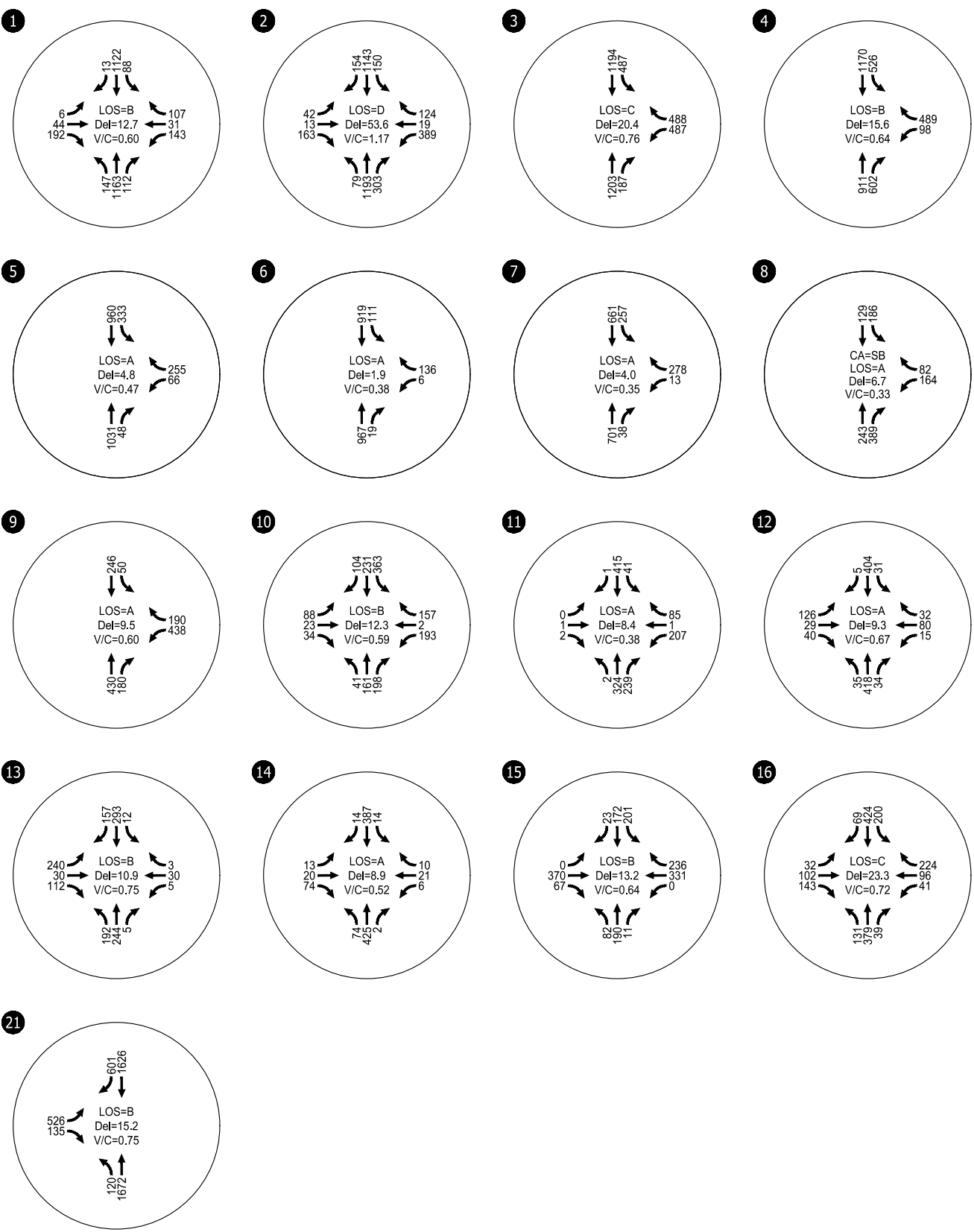
Year 2025 Background Traffic Conditions Saturday Midday Peak Hour Oregon City, Oregon
