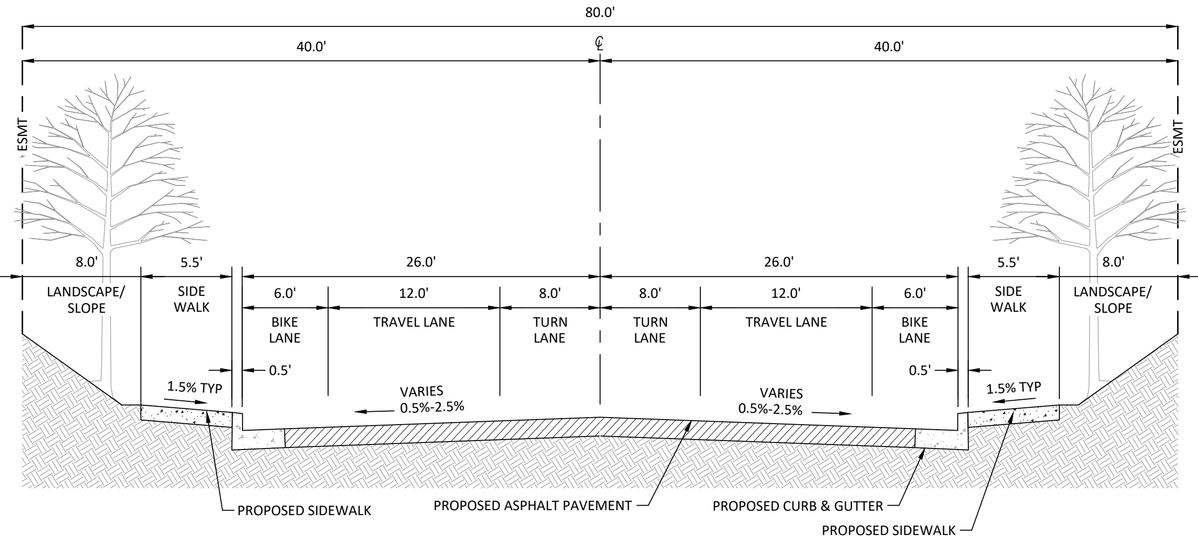
MARKET STREET (SECTION 1) N.T.S.
