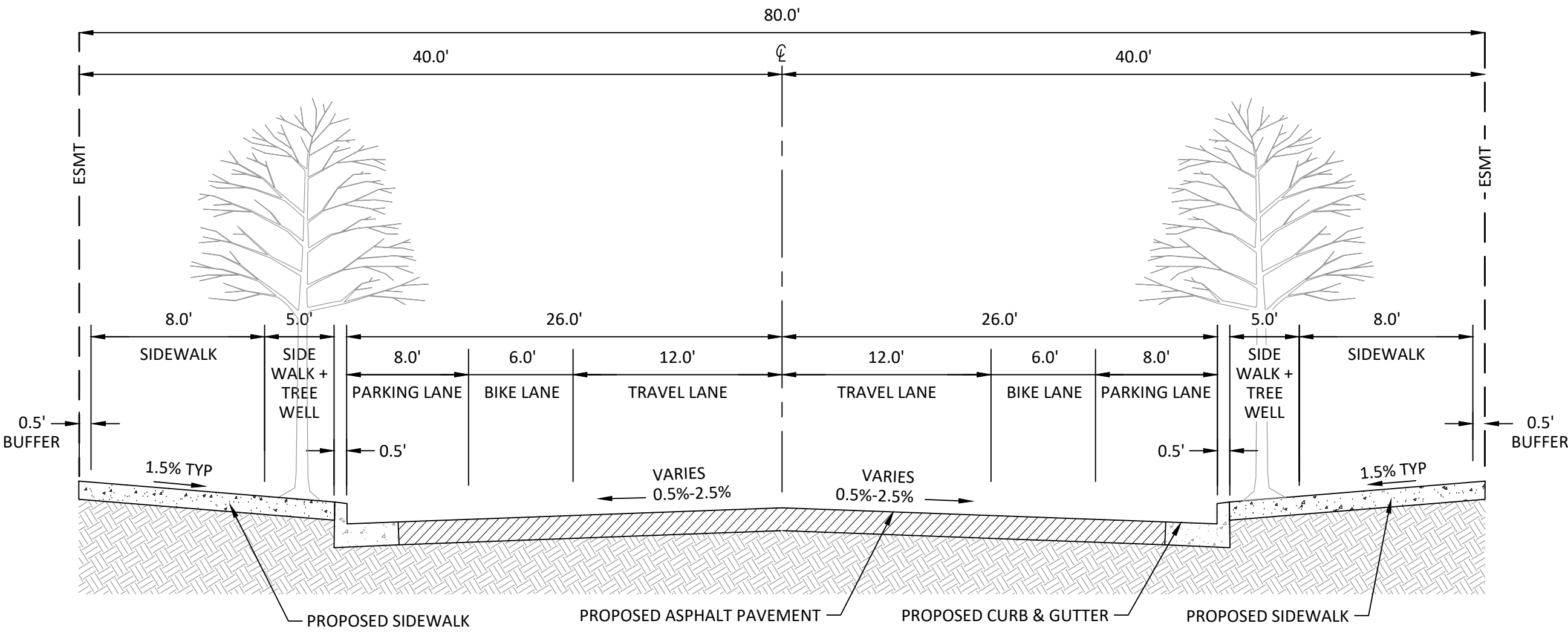
MARKET STREET (SECTION 2) N.T.S.
