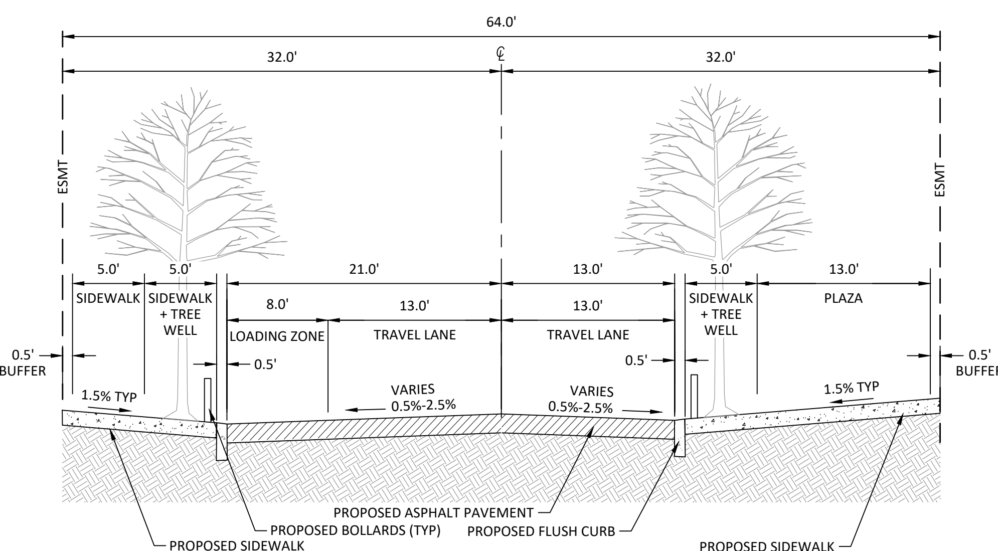
PLAZA FIRE ACCESS ROAD N.T.S.
