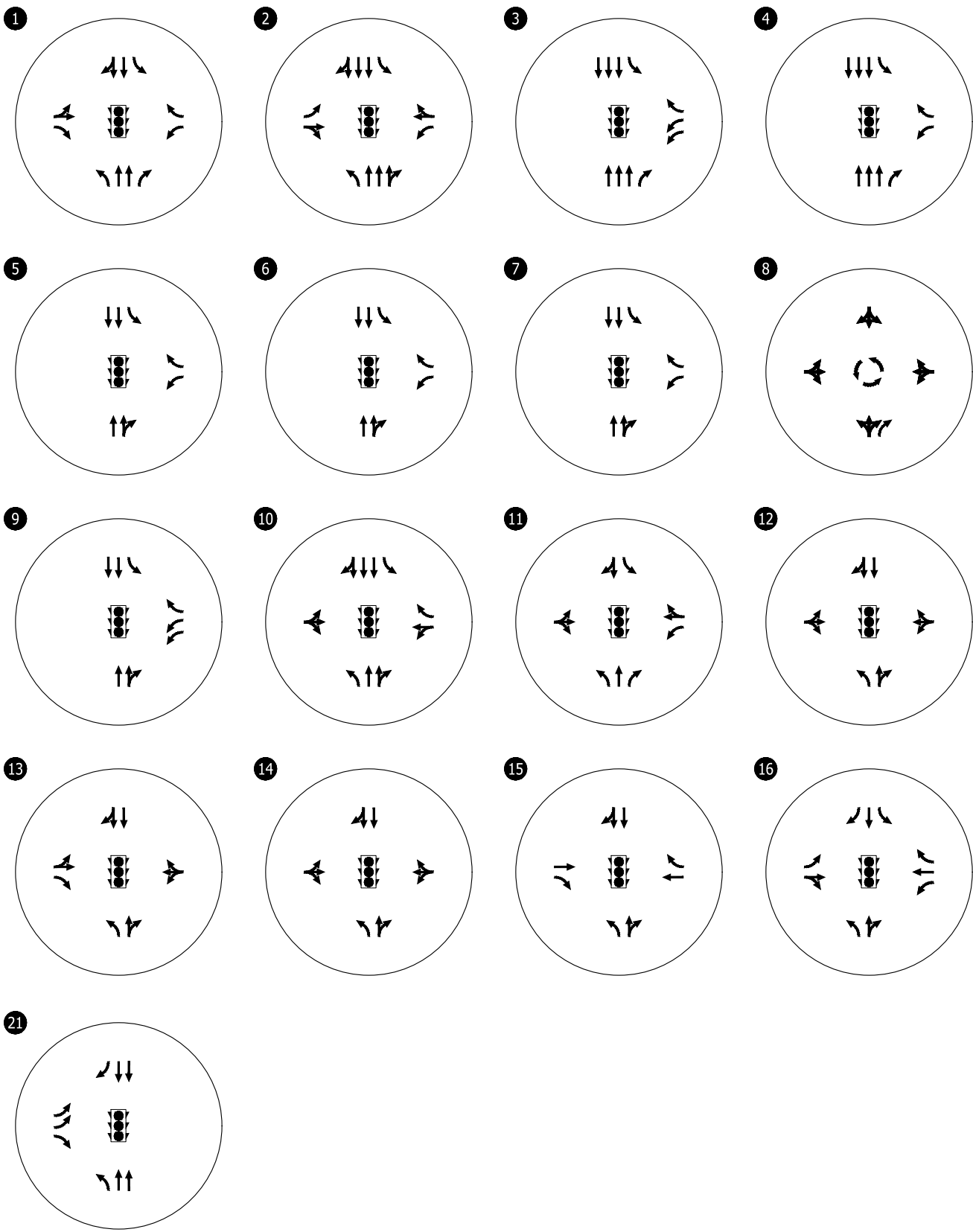
Existing Lane Configurations & Traffic Control Devices Oregon City, Oregon
