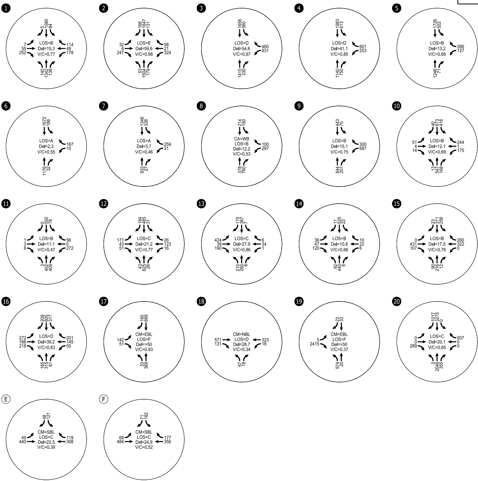
Year 2025 Total Traffic Conditions Weekday PM Peak Hour Oregon City, Oregon
