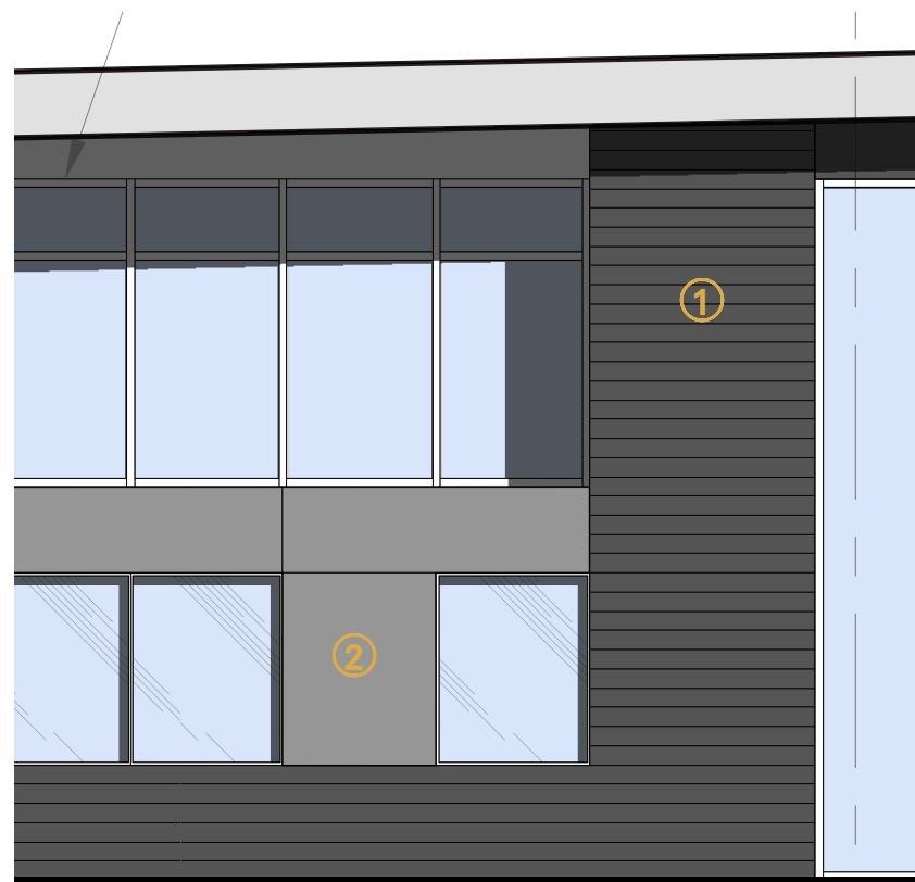
ENLARGED SOUTH FACADE
